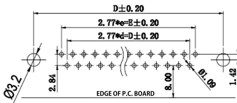
RECOMENDED P.C.B LAYOUT (TOP VIEW) TOLERANCES: \pm 0.05\text{mm}
